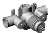
Ref. M00-2T7 Centrale thermostatique (55 l/min) Thermostatic mixer (55l/mn)
